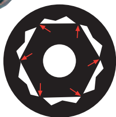
Conventional Spanner Surface Contact with a Fastener.
